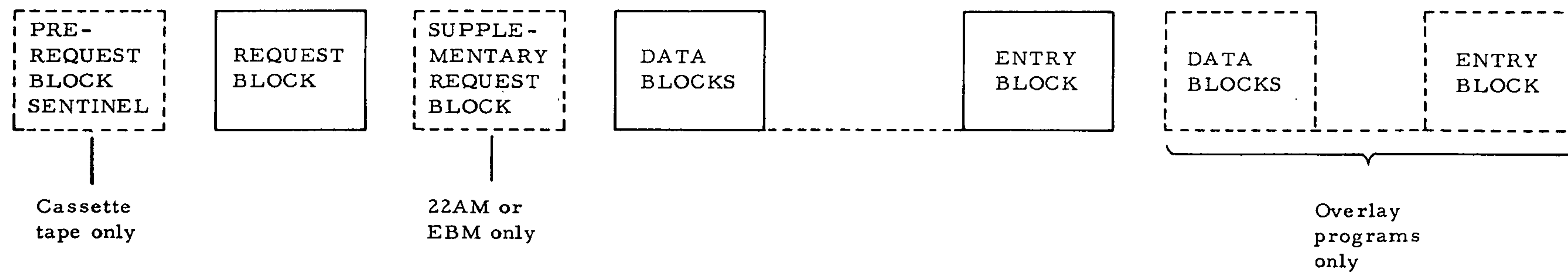
Figure 13 Format of a binary program
