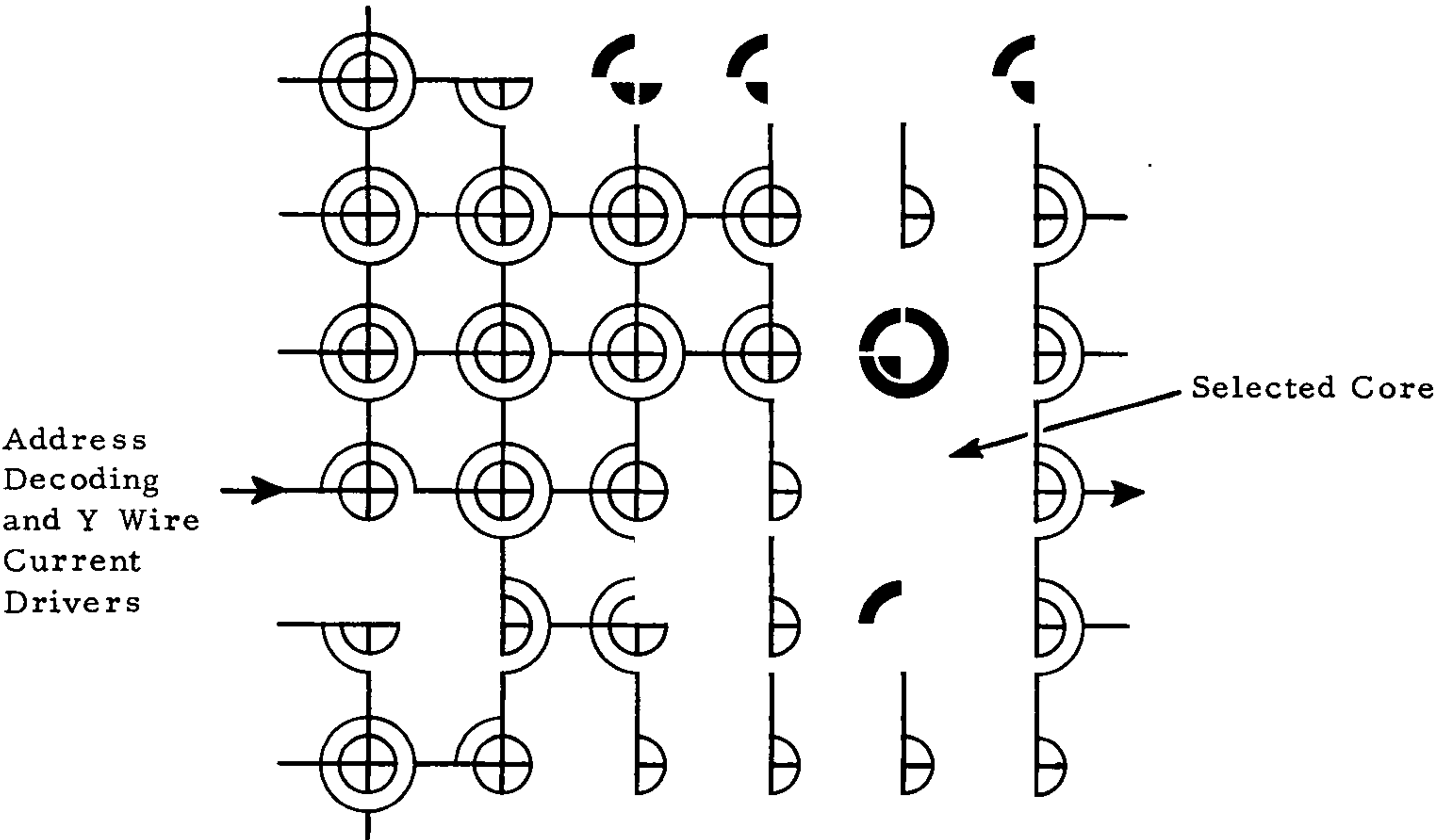
Address Decoding and X Wire Current Drivers
